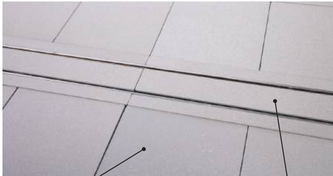
12x Pavement Sections 8-13/16 x 4-7/16 x 1/8" 22.4 x 11.2 x 0.4cm 6x Inner and Outer Track Walkways 8-13/16 x 1-5/16 x 1/16" 22.4 x 3.33 x 2cm
