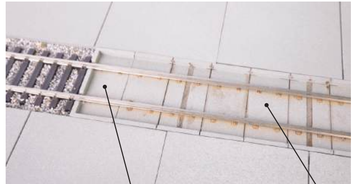
8x Cement Drip Pan End Sections 11/16 x 1-1/2 x 1/8" 1.8 x 3.8 x 0.4cm 12x Cement Drip Pan Center Sections 4-1/8 x 1-1/2 x 1/8" 10.5 x 3.8 x 0.4cm
